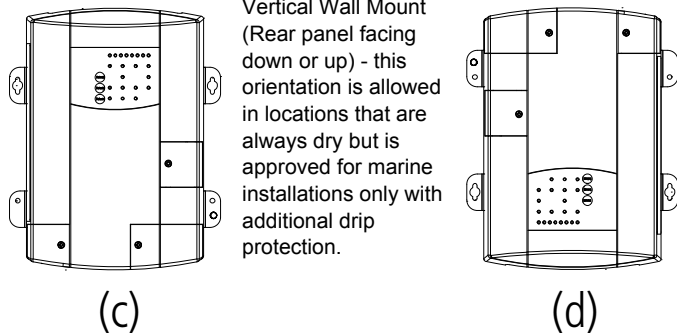
Figure 6 Mounting Orientations (Vertical)
