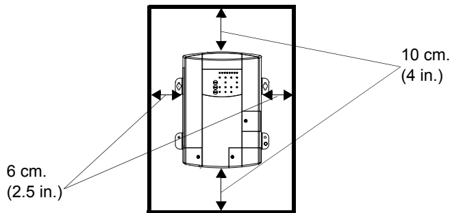
Figure 7 Ventilation Clearance
